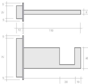
Polmet single bracket
