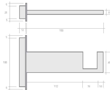
Polmet extended bracket
